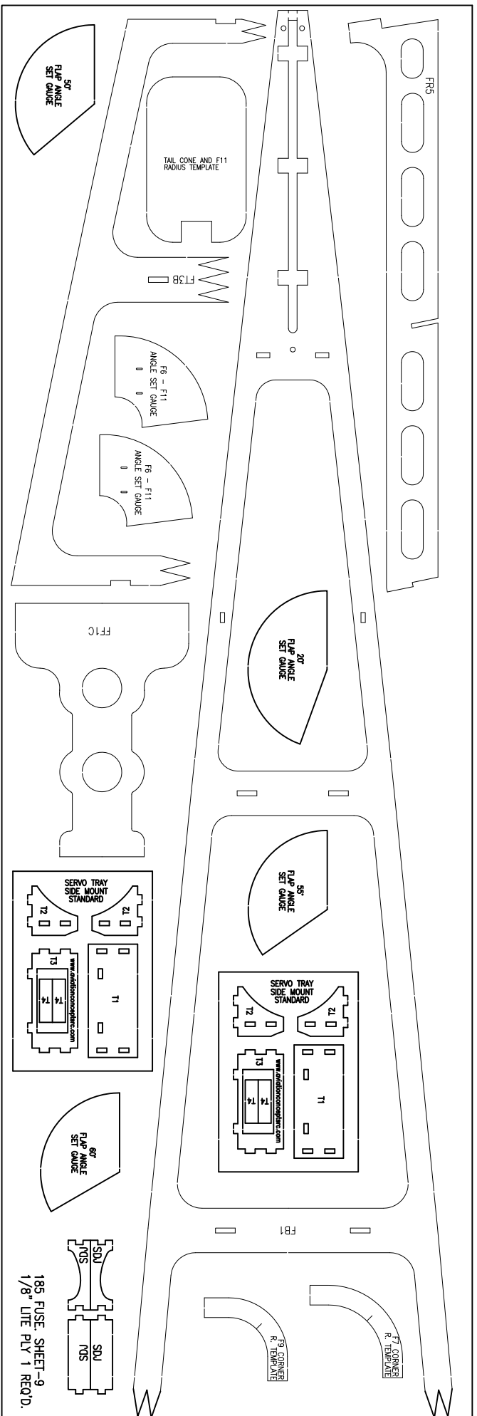
12" WIDE x 36" LONG x 1/8" THICK LITE PLY ONE (1) REQUIRED
