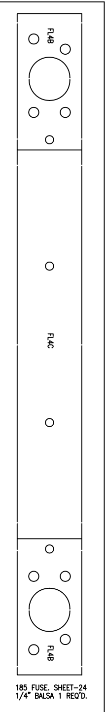
4" WIDE x 26" LONG x 1/4" THICK BALSA ONE (1) REQUIRED
