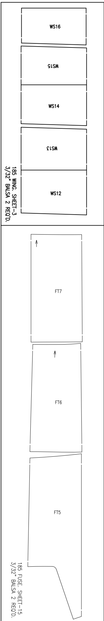
6" WIDE x 36" LONG x 3/32" THICK Balsa TWO (2) REQUIRED
